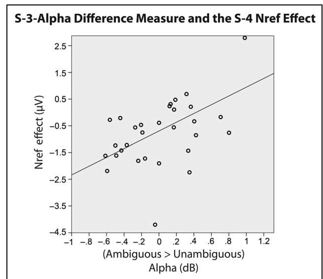
Figure 3. Single regression correlation between the S-3 alpha difference measure and the S-4 Nref effect. On the y axis is the S-4 Nref effect; on the x axis is the ambiguous > unambiguous S-3 difference in the alpha frequency band. Note that larger negative values for the Nref effect indicate larger effect sizes.
