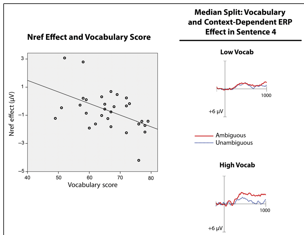
Figure 5. (Left) Single regression correlation between vocabulary score and the S-4 Nref effect. On the y axis is the S-4 Nref effect; on the x axis is the vocabulary score. Note that larger negative values for the Nref effect indicate larger effect sizes. (Right) For display purposes only, participants were split into high vocabulary ( N = 14 ) and low vocabulary ( N = 14 ) groups based on the median score (scores at the median were discarded). S-4 ERP results from the left-anterior electrode cluster, comparing ambiguous (solid red line) with unambiguous (dotted blue line) referents, are shown for the high vocab group (top) and the low vocab group (bottom).
