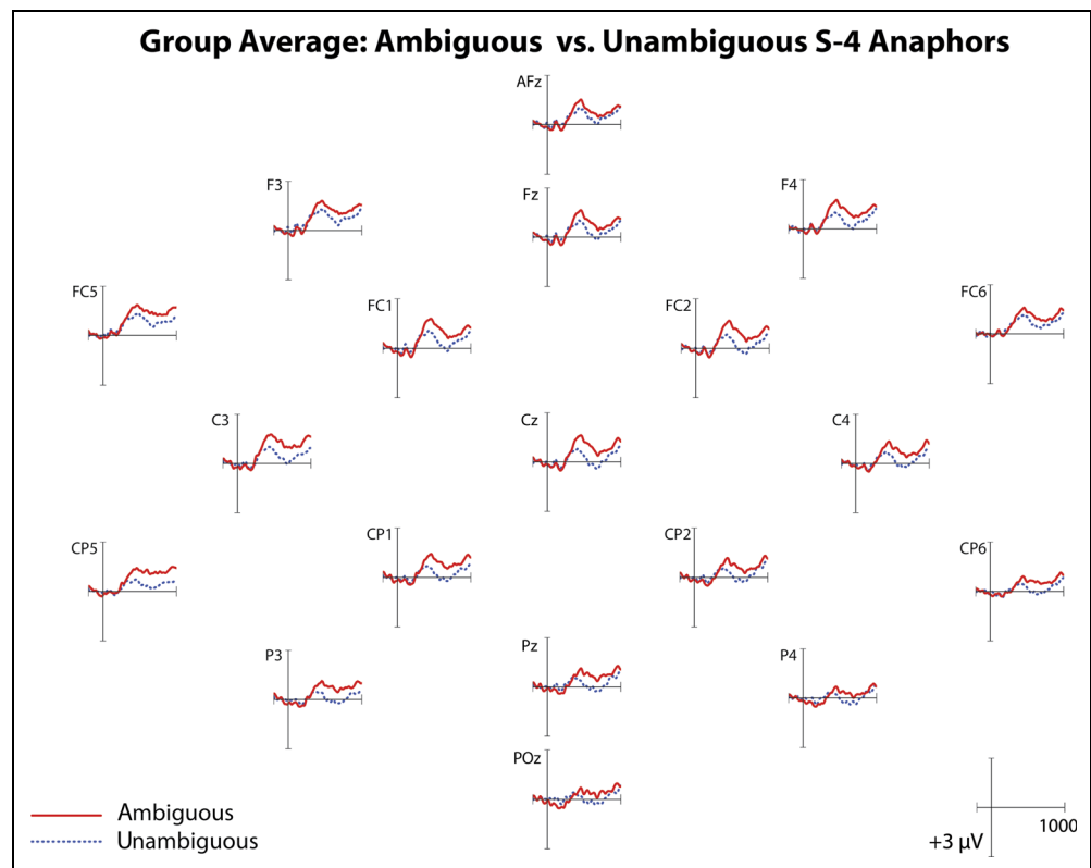
Figure 1. ERPs to the critical anaphor in S-4, comparing ambiguous (solid red line) with unambiguous (dotted blue line) anaphors. Negative is plotted up.
