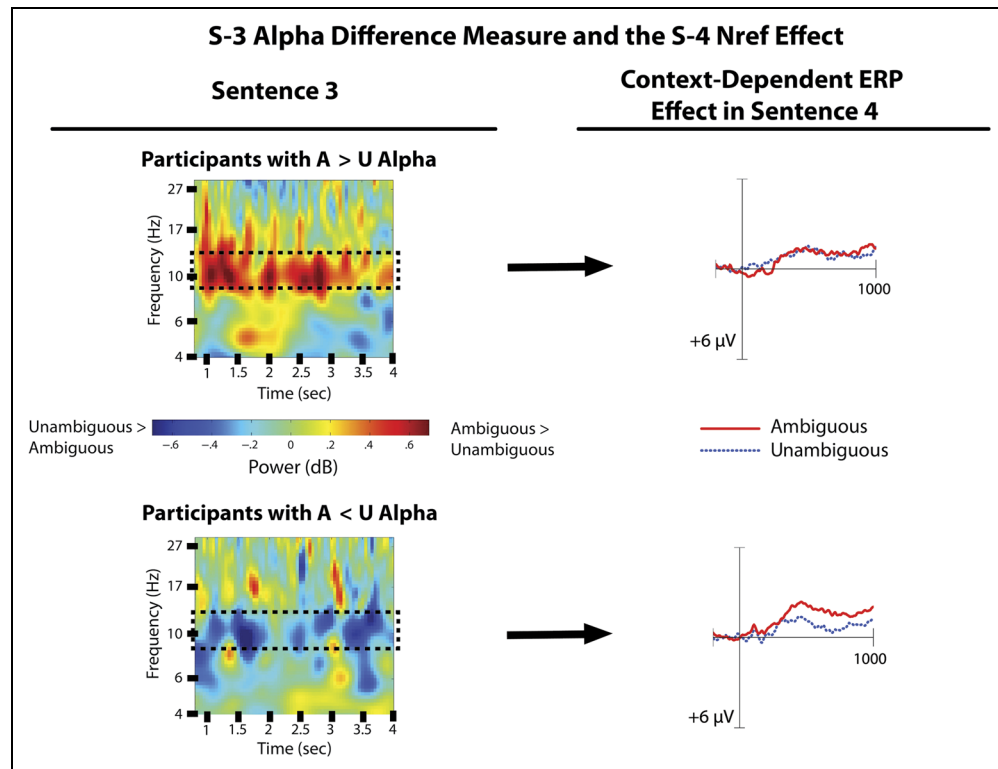
Figure 4. Relation between S-3 ambiguous > unambiguous alpha difference and S-4 Nref effect. For display purposes only, participants were split into A > U ( N = 16 ) and A < U ( N = 16 ) groups based on the median S-3 alpha difference value ( \sim 0 ). On the left are time-frequency plots showing spectral power for the S-3 difference across all frequencies examined; the alpha frequency band (9–12 Hz) is highlighted within the black boxes for the A > U group (top) and the A < U group (bottom). On the right are the corresponding S-4 ERP results from a representative electrode in the left-anterior electrode cluster (FC5), comparing ambiguous (solid red line) with unambiguous (dotted blue line) S-4 anaphors for the A > U group (top) and the A < U group (bottom).
